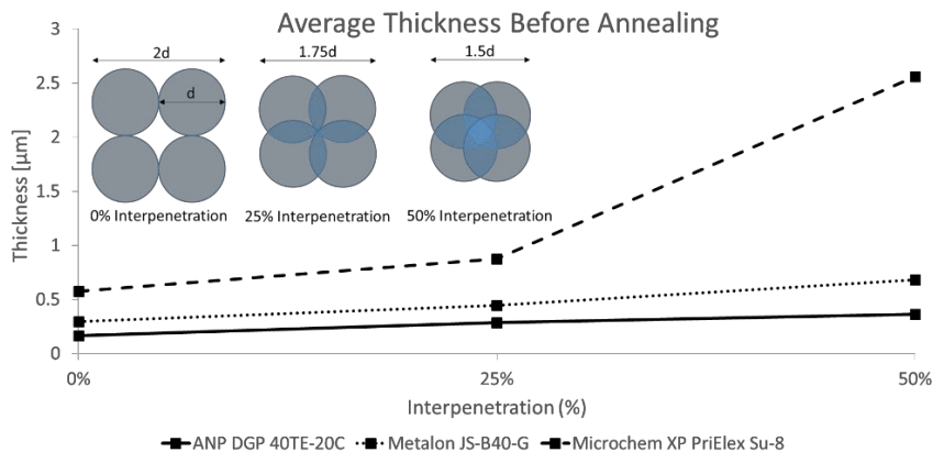
Figure 3 Effects of the interpenetration of the ink drops on the average thickness of the printed layers before any post-printing processes. Inset: Diagram of the layout of the ink drops with different interpenetration parameters.
