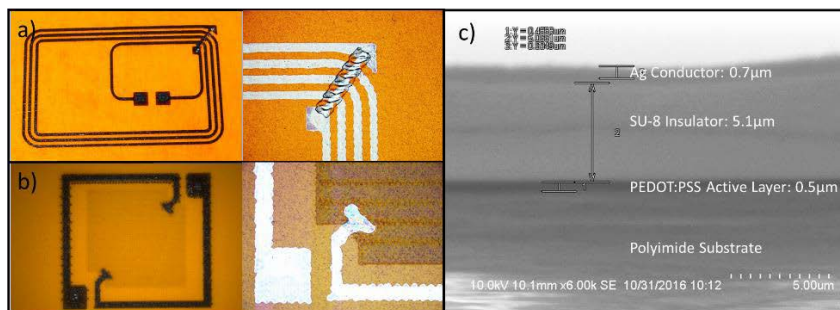
Figure 7 Three fully inkjet-printed device architectures. a) An antenna achitecture comprising of Ag/Su-8/Ag layers. b) A thermistor structure comprising of Ag/PEDOT:PSS layers. c) SEM image of a generic multilayered structure comprising of Ag/SU-8/PEDOT:PSS layers.
