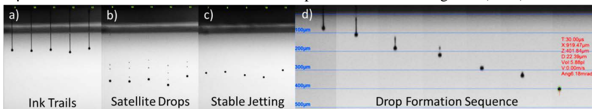
Figure 1 Inkjet drop analysis images taken with stroboscopic camera on CERADROP F-Series printer using ANP DGP 40TE-20C ink in Dimatix 1pL cartridge. a) Waveform used: 50V-3µs showing elongated ink trails. b) Waveform used: 35V-3µs showing few satellite drops at jetting distance. c) Waveform used: 22V-6µs showing stable drops at jetting distance. d) Waveform used: 22V-6µs showing stable drop formation.
